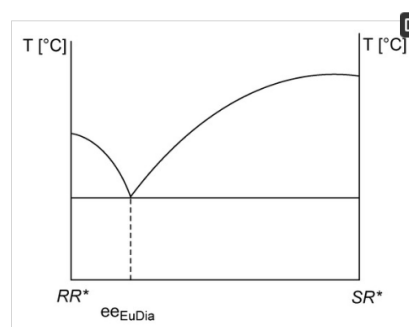
Figure 2. Binary melting phase diagram of a diastereomeric mixture of RR^* and SR^* [3,6] and the possibility of calculating the achievable F value using the ee_{Dia} (Equation (2)).
